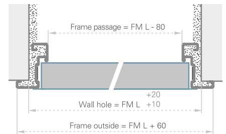
ONE LEAF DOOR - HORIZONTAL SECTION
