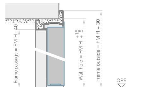
DOOR WITHOUT BOTTOM STOP - VERTICAL SECTION
