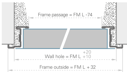
ONE LEAF DOOR - HORIZONTAL SECTION
