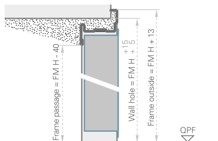
DOOR WITHOUT BOTTOM STOP - VERTICAL SECTION
